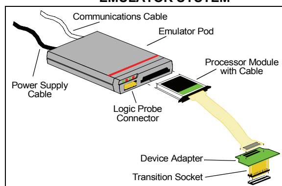
FIGURE 2-1: MPLAB ® ICE 2000 EMULATOR SYSTEM
